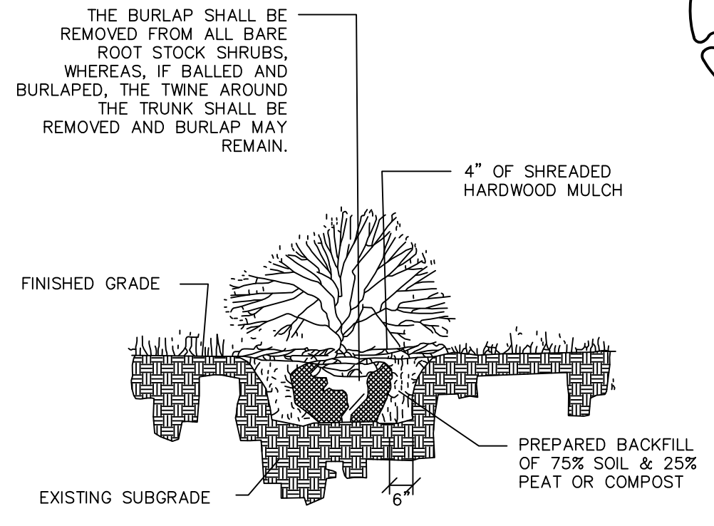
SHRUB DETAIL N.T.S.
