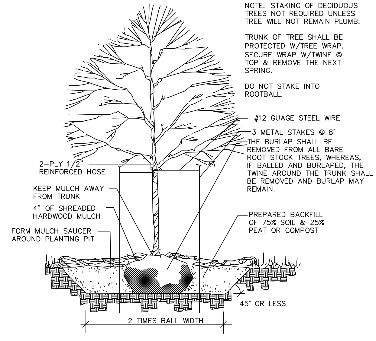
DECIDUOUS TREE DETAIL N.T.S.
