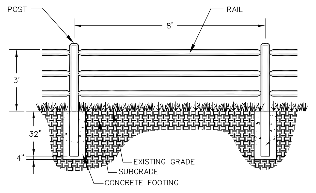
ROUND RAIL FENCE DETAIL N.T.S.
